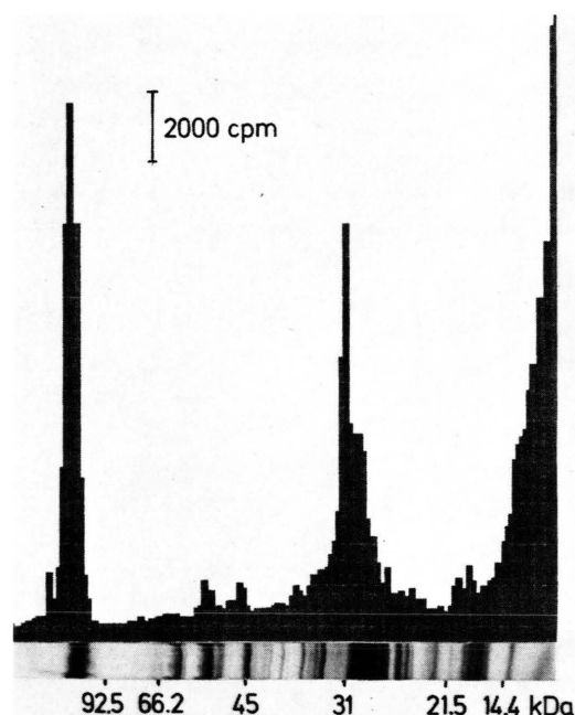
Fig. 3. Photograph and radioactivity scan of a LDS polyacrylamide gel (10–15%) of thylakoids labeled by 7.5 nmol/mg Chl [ ^{125}\text{I} ] TID. The molecular weight numbers indicate the positions of the marker proteins.
