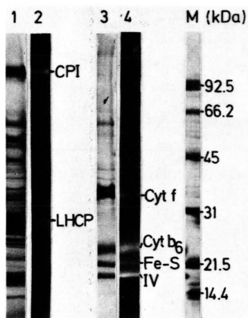
Fig. 2. Photographs (1, 3) and autoradiograms (2, 4) of LDS-polyacrylamide gels (10–15%) of thylakoids (1, 2) labeled by 7.5 nmol/mg Chl and cytochrome b_6/f -complex (3, 4) labeled by 1.2 nmol/nmol cytochrome f [ ^{125}\text{I} ] TID. M = marker proteins.
