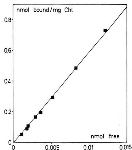
Fig. 1. Binding of [ 125 I] TID to thylakoid membranes. For conditions, see Materials and Methods.
